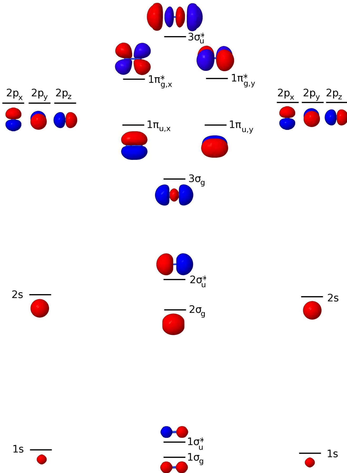
Figure 1: Molecular Orbital Diagram for a Homonuclear Diatomic Molecule.
